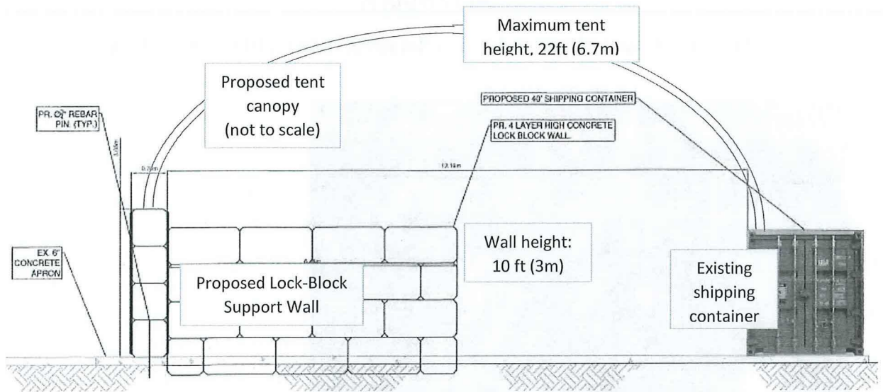
Figure 3: Illustration of proposed tent and support structure – front view, facing Recycling Depot parking area
