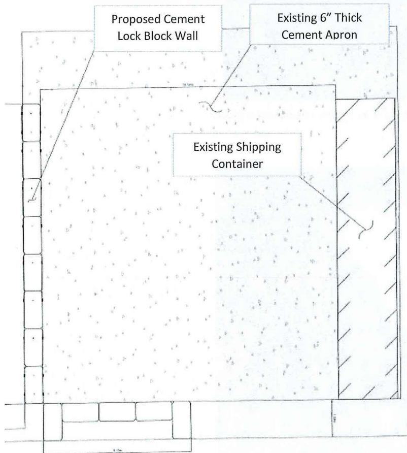
Figure 4 – Illustration of proposed 40' x 40' support structure - plan view
