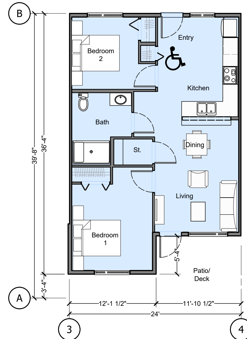
Unit Type C4 Accessible 2 Bedroom 810 sq.ft.
