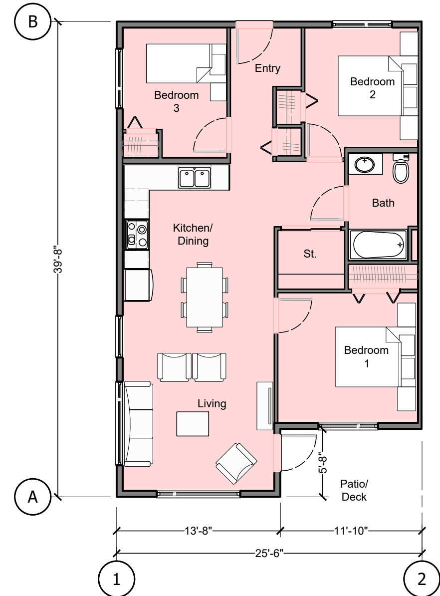
Unit Type D1 Adaptable 3 Bedroom 944 sq.ft.
