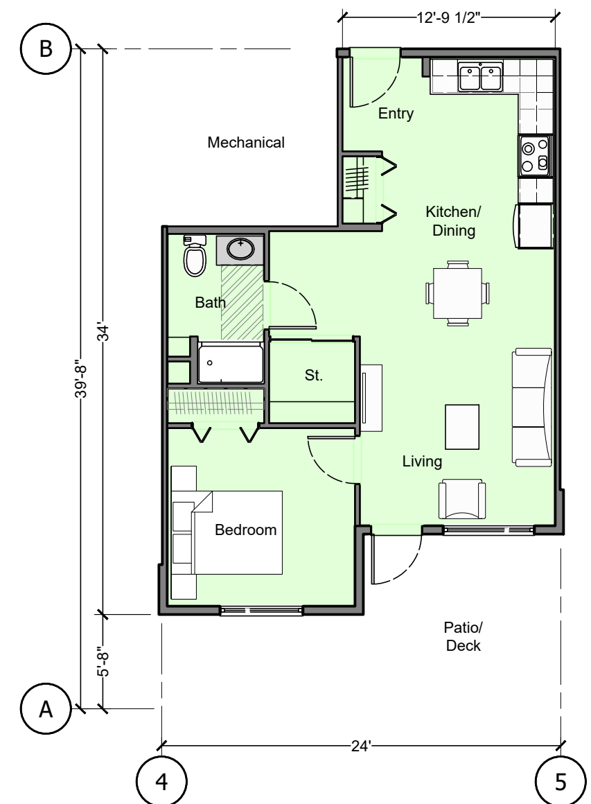
Unit Type B4 Adaptable 1 Bedroom 648 sq.ft.
